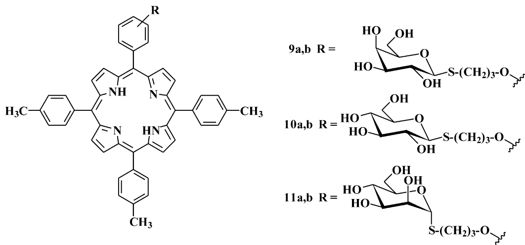
Figure 1. Structures of thioglycosylated meso porphyrins. a and b refer to ortho and para positions, respectively.
